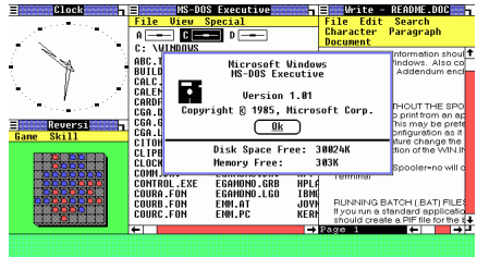
(b) Windows
