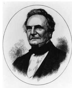
(b) Babbage
