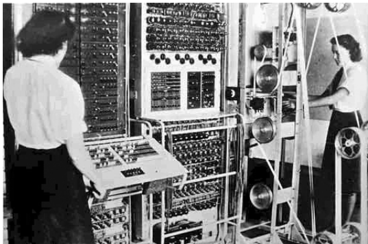
(b) COLOSSUS
